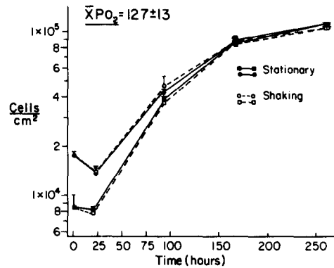
FIGURE 5. Shaken vs. stationary growth of human diploid fibroblasts inoculated at 10^4 or 2 \times 10^4 cells/cm 2 at PO 2 127 mm Hg. Shaken cells were tilted through a 60° arc every 5 s. Each point represents the mean \pm SD of three flasks. The error bars indicate the standard deviation. Three flasks at each seeding density were shaken for the first 24 h and harvested at 24 h. The remainder of the shaken flasks were incubated stationary for 24 h and placed on the rocking platform at 24 h. (□, ■) Inoculated at 1 \times 10^4 cells/cm 2 ; (○, ●) inoculated at 2 \times 10^4 cells/cm 2 .
